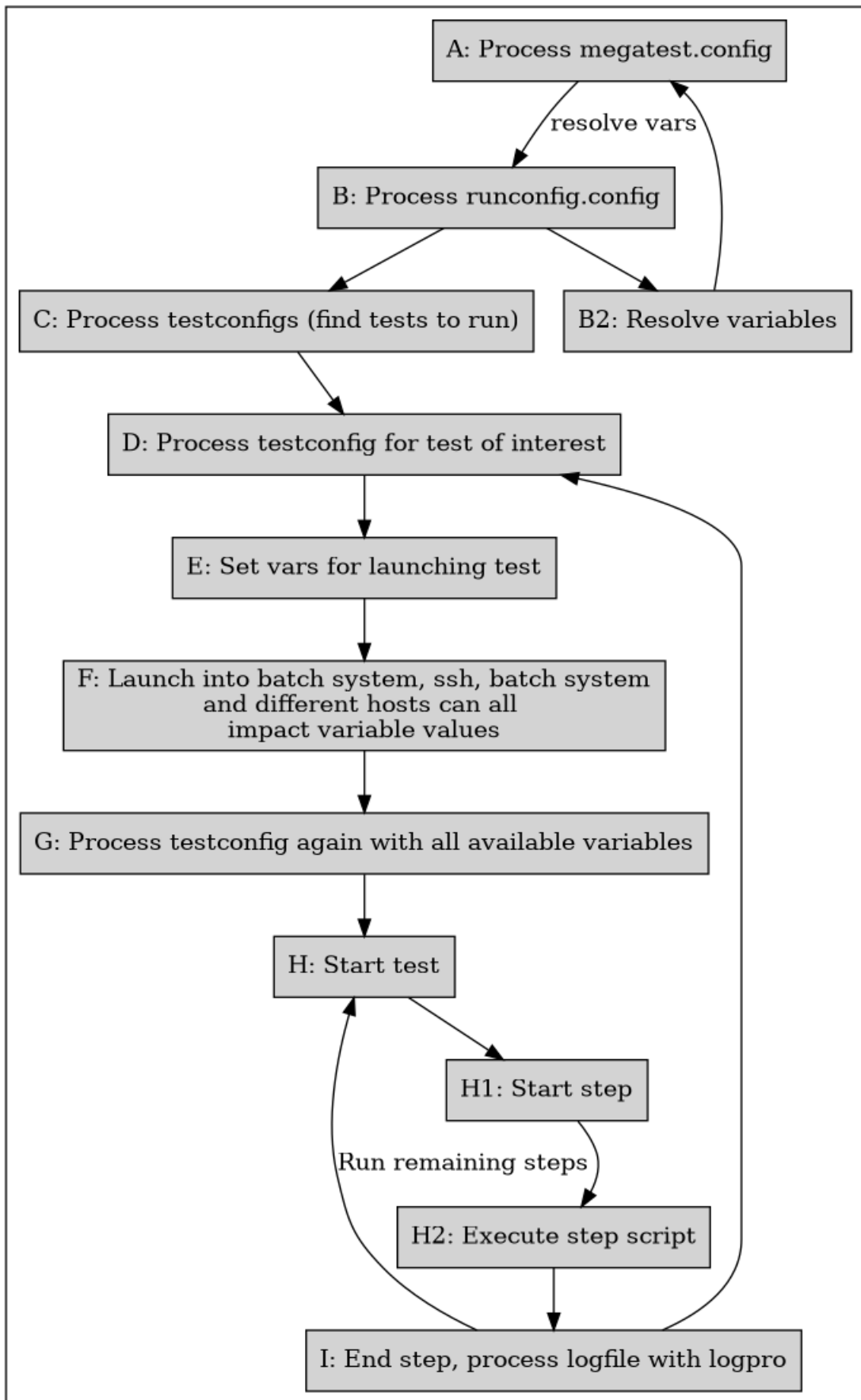
Figure 11.2: A simplified diagram of the stages Megatest goes through to run a test.
